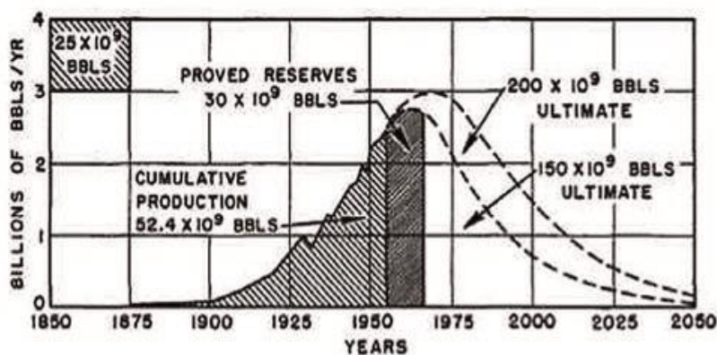
Figure 21 - Ultimate United States crude-oil production based on assumed initial reserves of 150 and 200 billion barrels.
